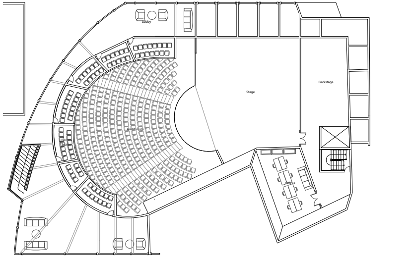
Floor Plans
